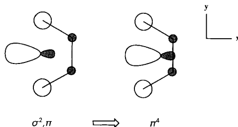
Fig. 4. Dominating orbital contributions to the back bonding interaction between butadiene and [Zr(allyl)Cp] fragment orbitals
