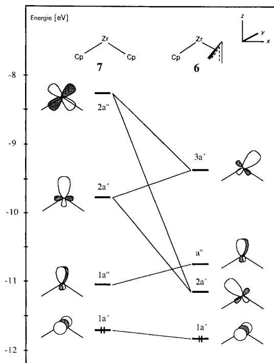
Fig. 1. A correlation of the valence orbitals of a [\text{ZrCp}_2] ( 7 ) and a [\text{Zr}(\text{allyl})\text{Cp}] ( 6 ) fragment
