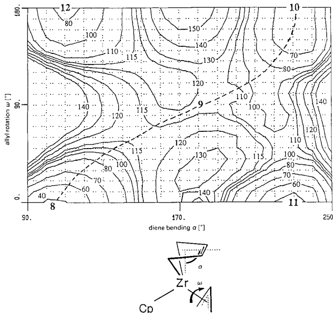
Fig. 5. Energy contour plot of the optimized geometries of the simultaneous allyl rotation and diene inversion 8 \leftrightarrow 10 (energies in kJ/mol with respect to the fully optimized structure 3a )
