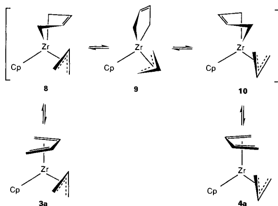
Scheme 2. Proposed Pathway for the Rearrangement of the Diene and Allyl Ligand from 3a to 4a
