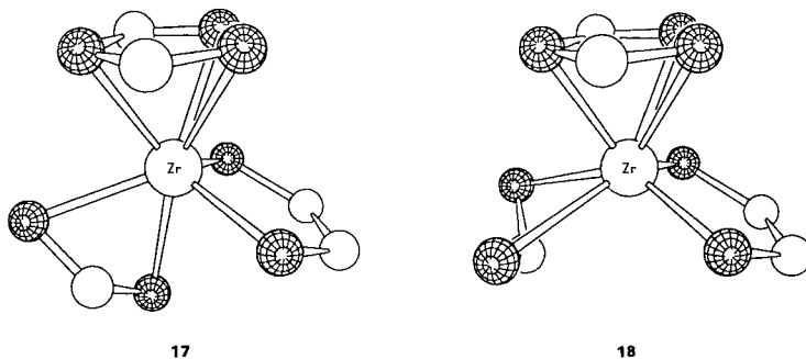
Fig. 7. Simplified representation of 9 and 14 as [\text{ML}_7] species
