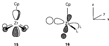
Fig. 6. Orbital representations of the decisive functions in 13a and 13b
