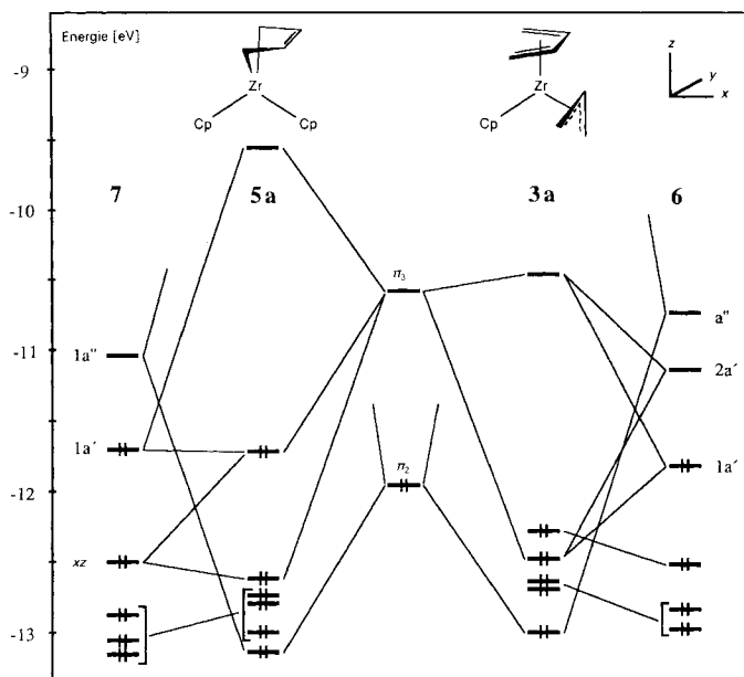
Fig. 2. MO-Interaction scheme of butadiene and [ZrCp_2] ( 7 ) and [Zr(allyl)Cp] ( 6 ) fragment orbitals
