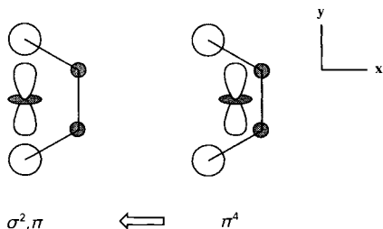
Fig. 3. Dominating orbital contributions to the HOMO in 5a
